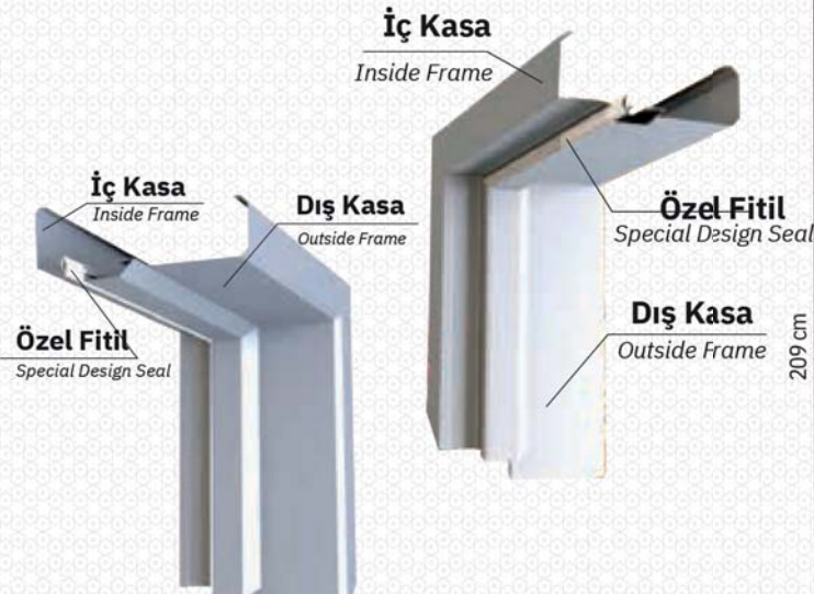
Kasa Kesit / Frame Details
